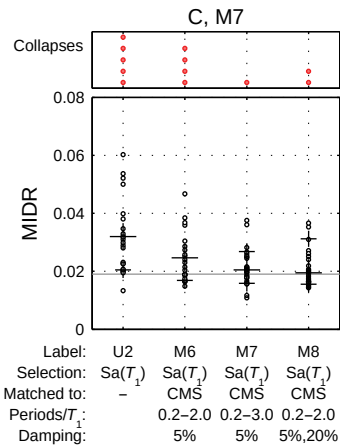
Figure B-13 Comparison of maximum interstory drift ratios showing Suite U2 (unmatched), Suite M6, Suite M7, and Suite M8 (matched to Conditional Mean Spectrum with different period range and damping ranges).
